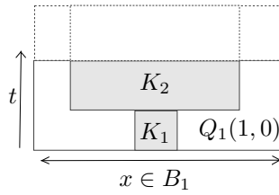
Figure 4: A supersolution in a smaller cylinder.
