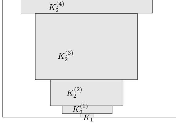
Figure 6: Stacks of neighbourhoods K_2^{(k)} .
