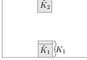
Figure 1: The two neighbourhoods \tilde{K}_1 and \tilde{K}_2 .
