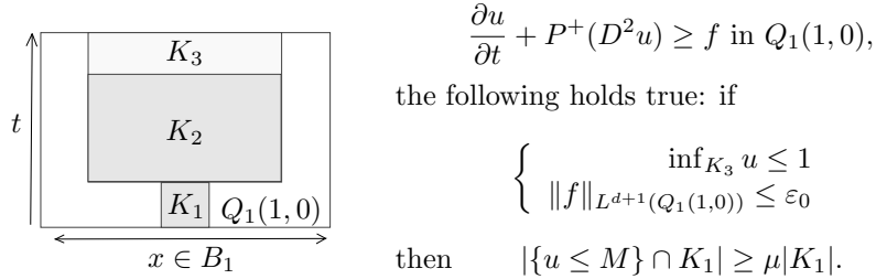
Figure 3: Basic measure estimate in Q_1(1,0) .
