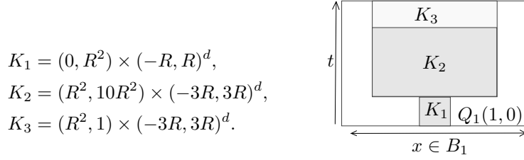
Figure 2: The sets K_1 , K_2 and K_3 .
