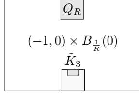
Figure 9: The set \tilde{K}_3 .
