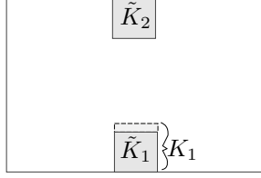
Figure 8: The two neighbourhoods \tilde{K}_1 and \tilde{K}_2 .
