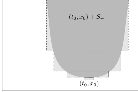
Figure 5: Stacks of cubes.
