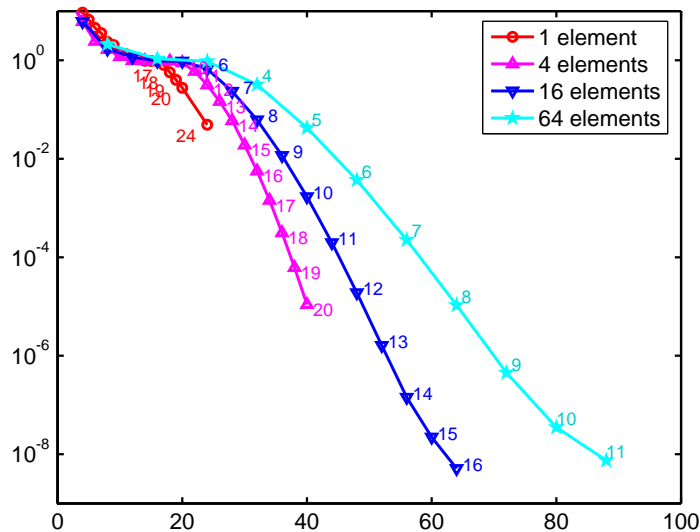
Figure 21: Relative errors for first eigenvalue, vs. number of Dof per side. Semi-logarithmic scale from 10^{-9} to 10 for errors. Integers mark polynomial degree.
