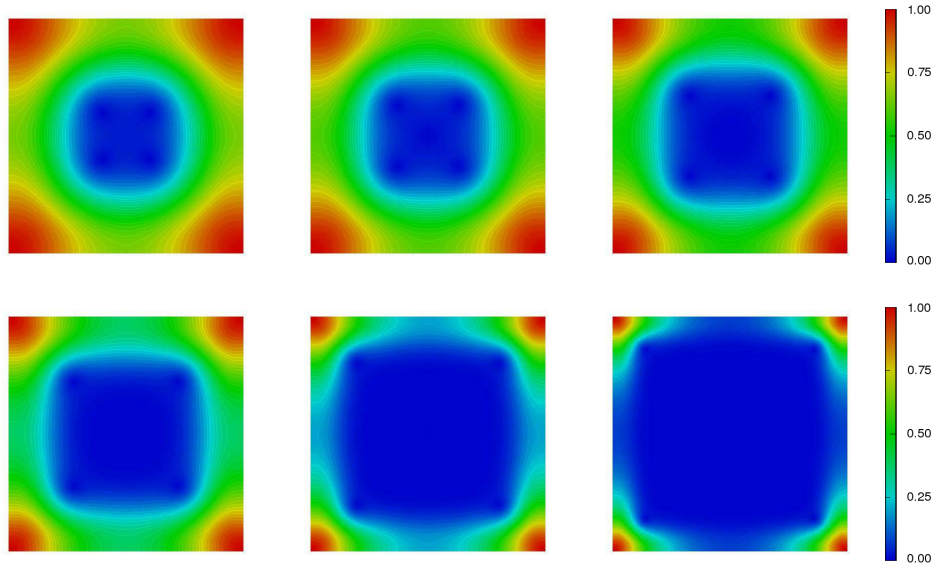
Figure 6: Moduli of the first eigenfunction, h = 0.1, 0.08, 0.06, 0.04, 0.02, 0.01 .
